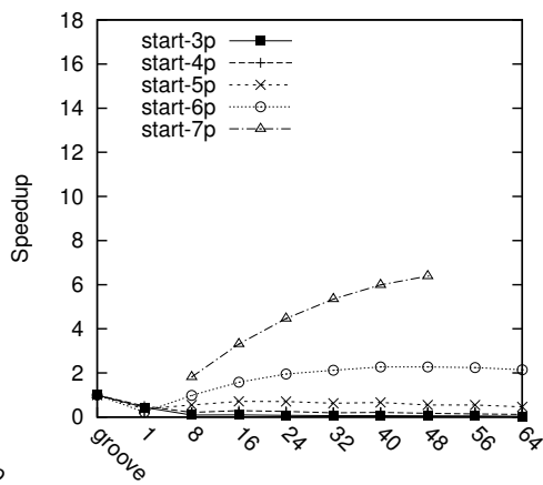
(f) 1e, enc_L . Speedup compared to GROOVE.
