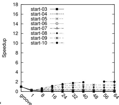
(f) unflagged-platoon, enc_L . Speedup compared to GROOVE.
