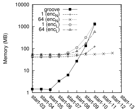
(b) unflagged-platoon. Memory usage for GROOVE and LTSMIN (per core).
