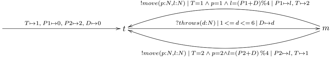
Figure 2.4: The IOSTS of a board game example
