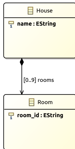
(b) Type Model Tm_5
