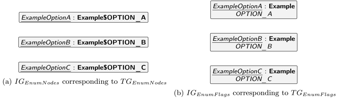
Figure 5.12: Visualisation of the transformation of enumeration values corresponding to an enumeration type
