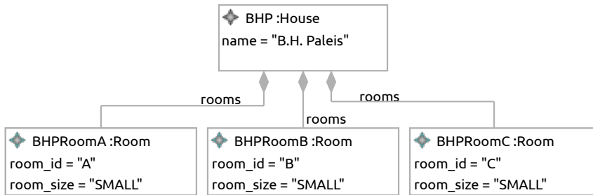
(a) Instance Model Im_7
