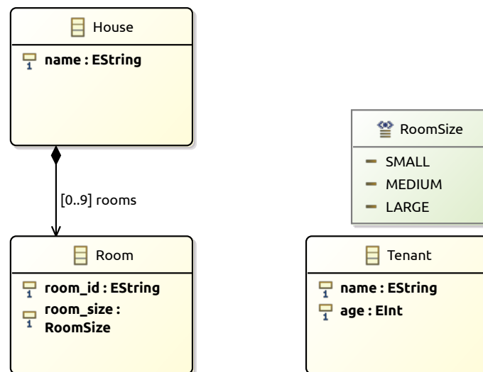
(b) Type Model Tm_{10}
