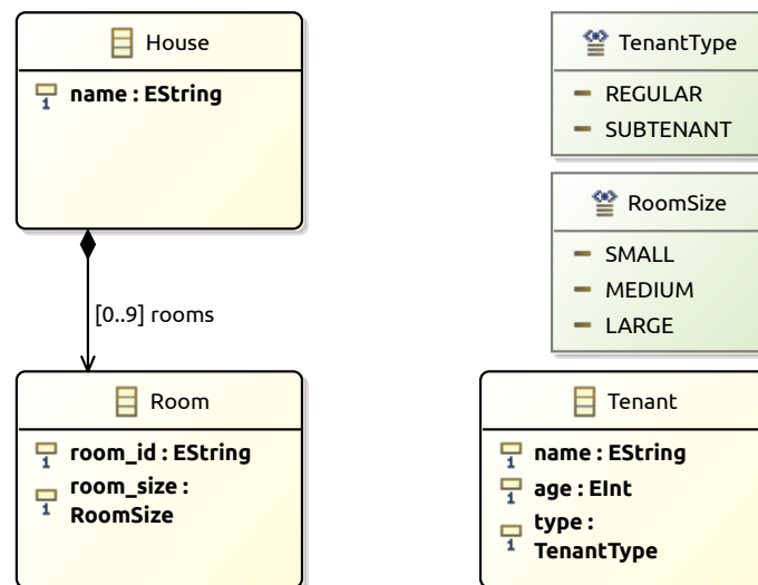
(b) Type Model Tm_{12}
