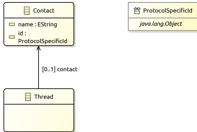
(b) The contact extension model Tm_{Extension}
