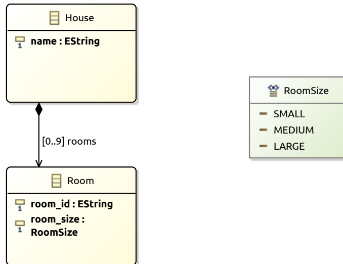
(b) Type Model Tm_7
