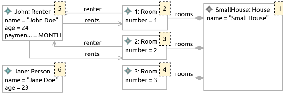
Figure 3.4: Model not satisfying the abstract property.
