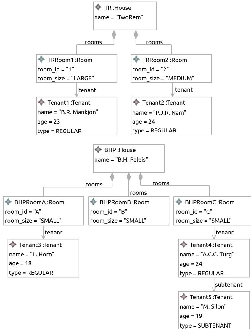
(a) Instance Model Im_{14}
