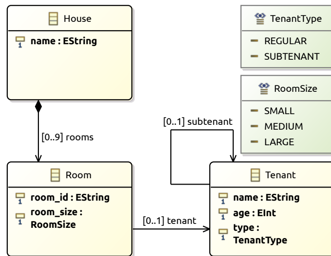
(b) Type Model Tm_{14}
