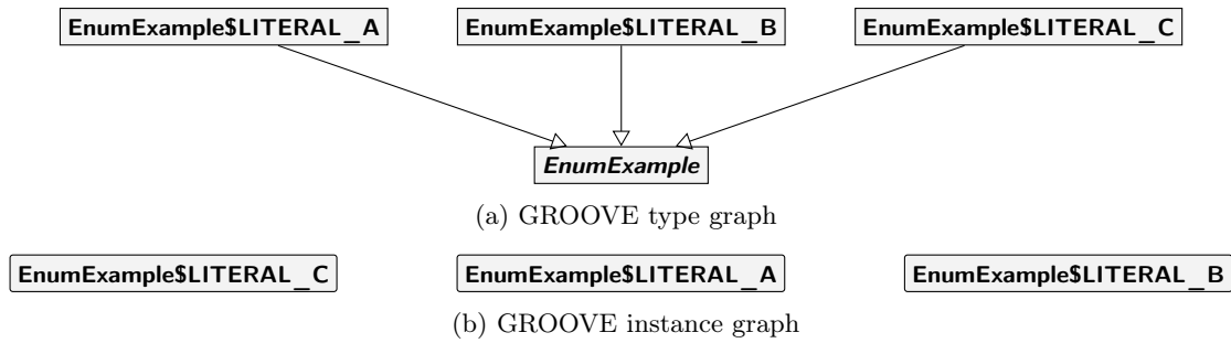
Figure 4.2: Encoding of the EnumExample enumeration type as different nodes types
