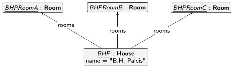
(a) Instance Graph IG_4
