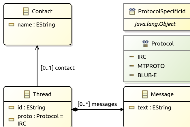
(c) The extended chat application model Tm_{ChatExt}
