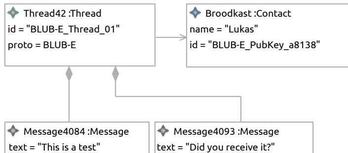
(c) The extended chat application instance model Im_{ChatExt}
