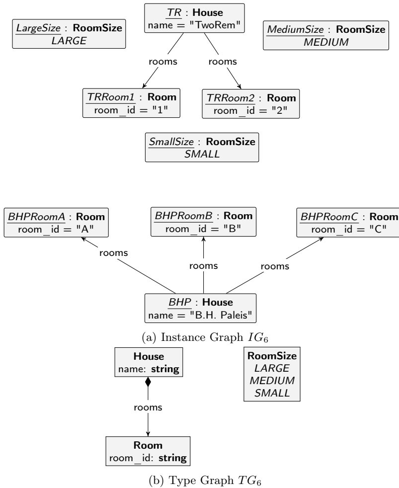
Figure 6.13: The GROOVE graphs after step 6
