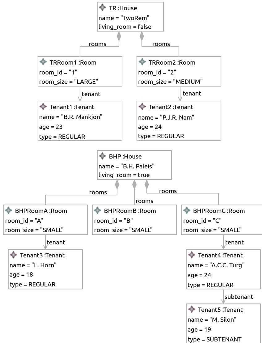
(a) Instance Model Im_{15}
