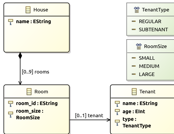
(b) Type Model Tm_{13}
