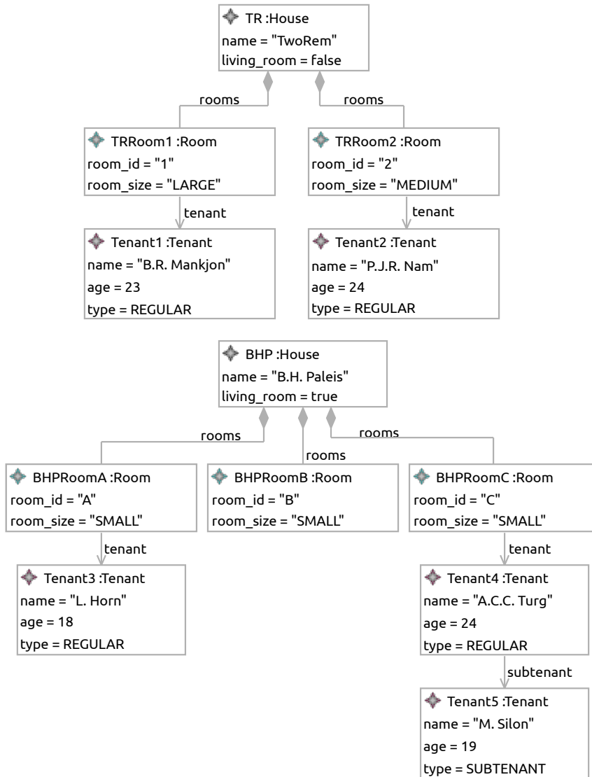
(a) Instance model
