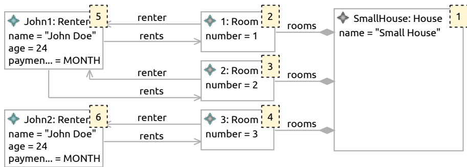
Figure 3.6: Model not satisfying the identity property.
