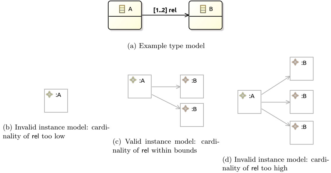
Figure 3.3: Examples of valid and invalid multiplicities
