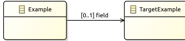
(a) Tm_{NullableClassField} to a class type .TargetExample with name = field
