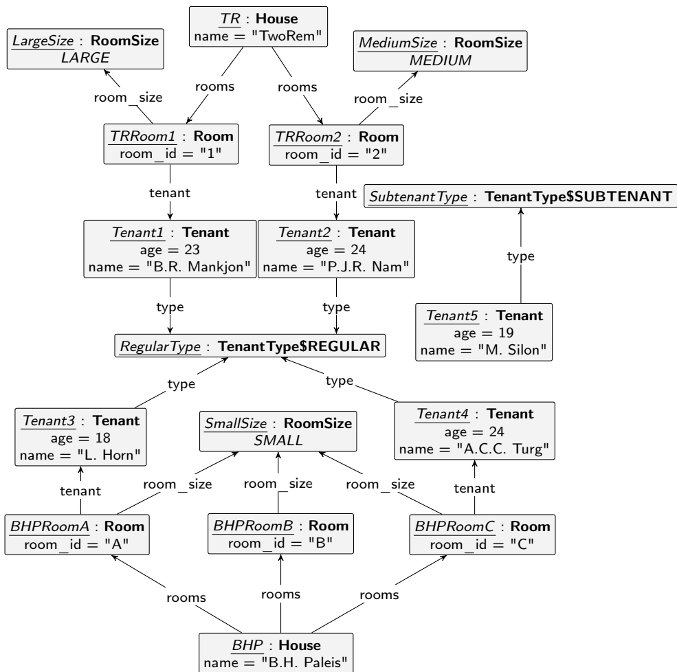
(a) Instance Graph IG_{13}
