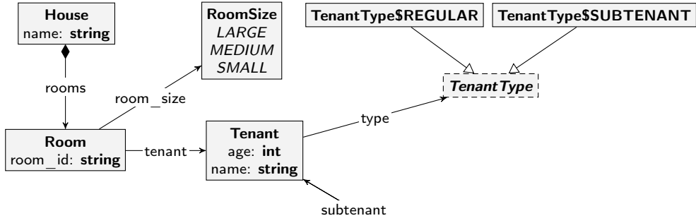
(b) Type Graph TG_{14}
