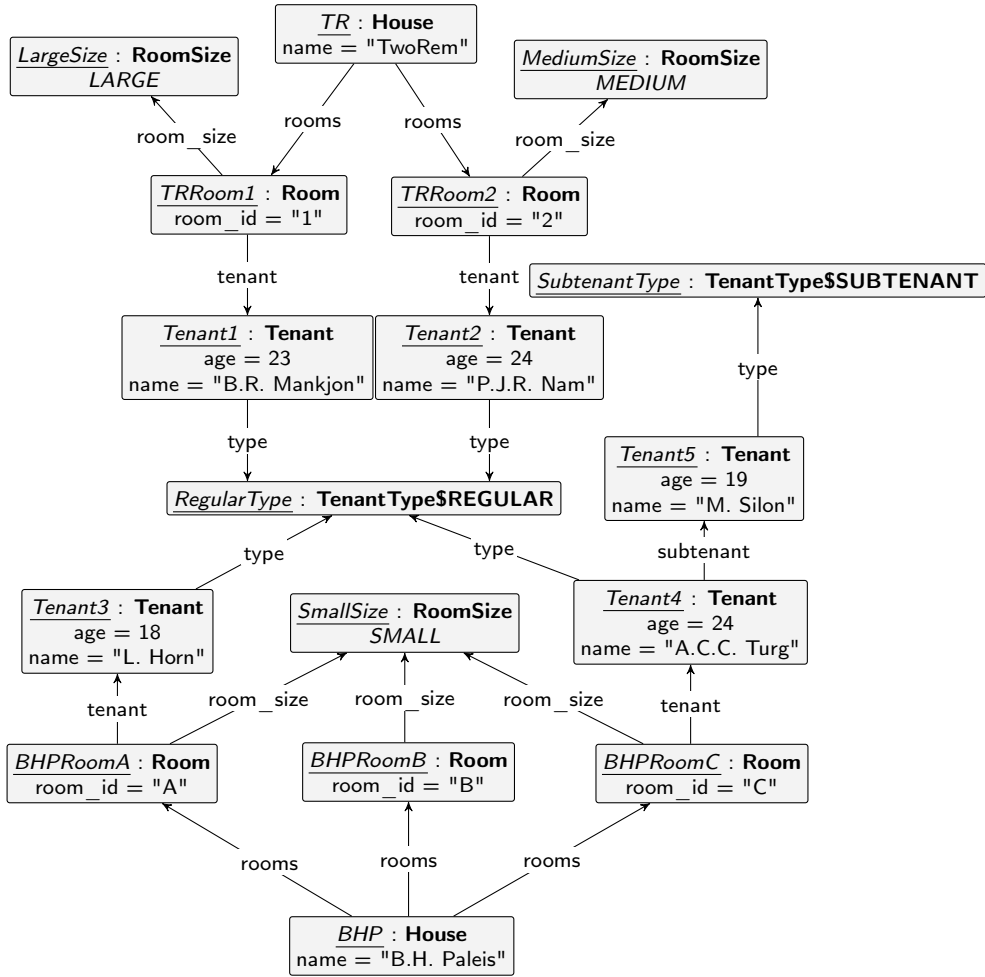
(a) Instance Graph IG_{14}
