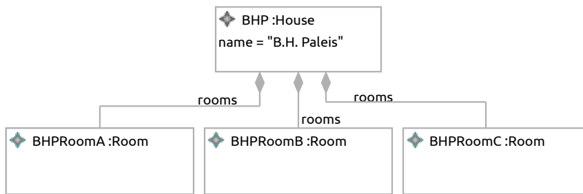
(a) Instance Model Im_4
