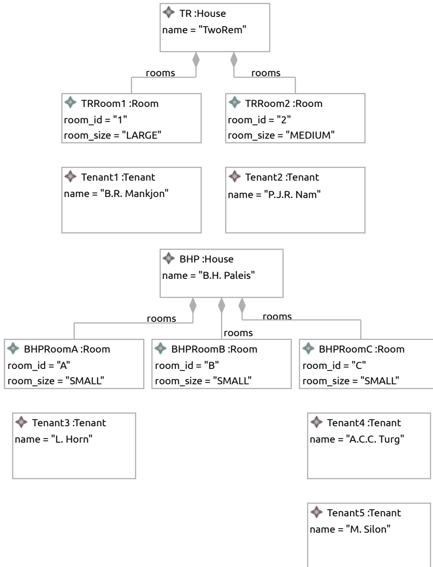
(a) Instance Model Im_9
