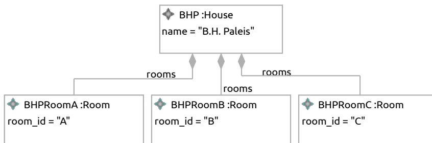
(a) Instance Model Im_6
