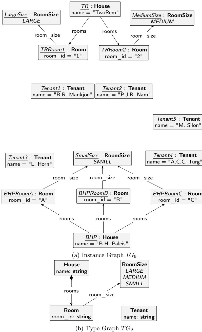
Figure 6.19: The GROOVE graphs after step 9
