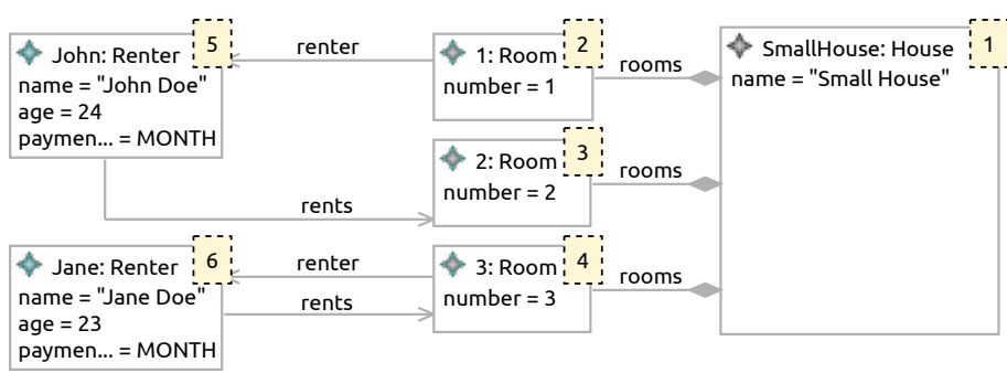
Figure 3.8: Model not satisfying the opposite property.
