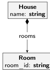
(b) Type Graph TG_5
