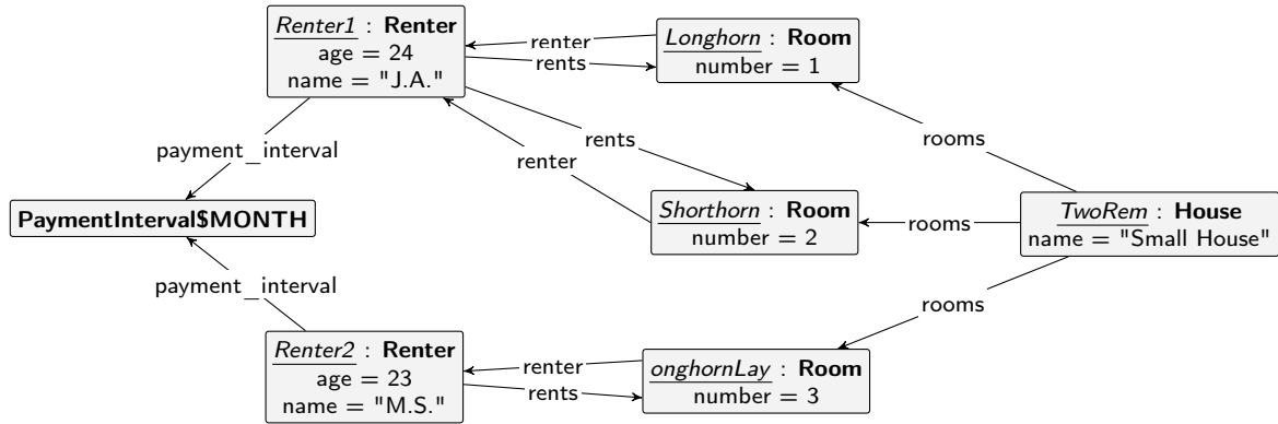
(a) Instance graph in GROOVE's visual notation
