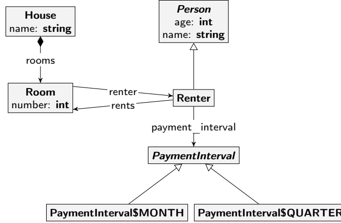
(a) Type graph in GROOVES visual notation. Multiplicities are omitted for clarity.
