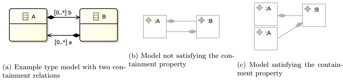
Figure 3.5: Examples of the containment property.
