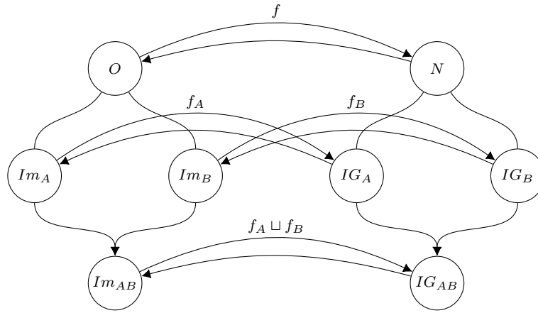
Figure 4.10: Structure for transforming between instance models and instance graphs
