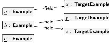
(b) IG_{ContainedClassSetField} with examples of different nodes with different values for field
