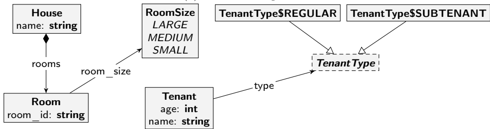
(b) Type Graph TG_{12}
