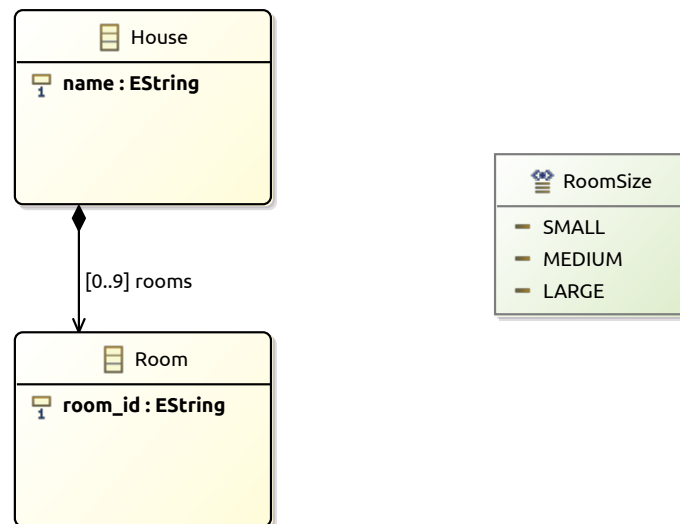
(b) Type Model Tm_6
