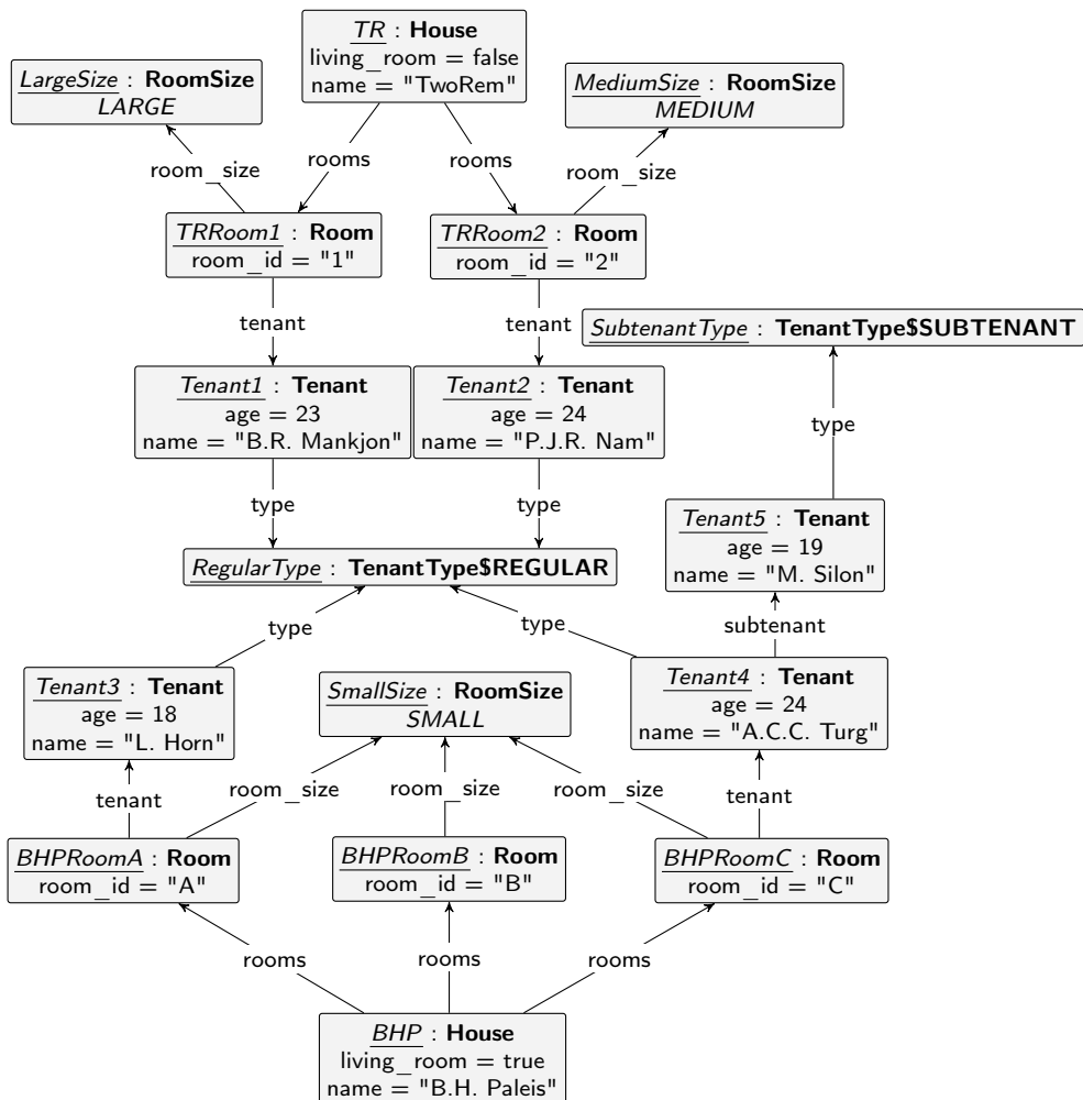
(a) Instance Graph IG_{15}
