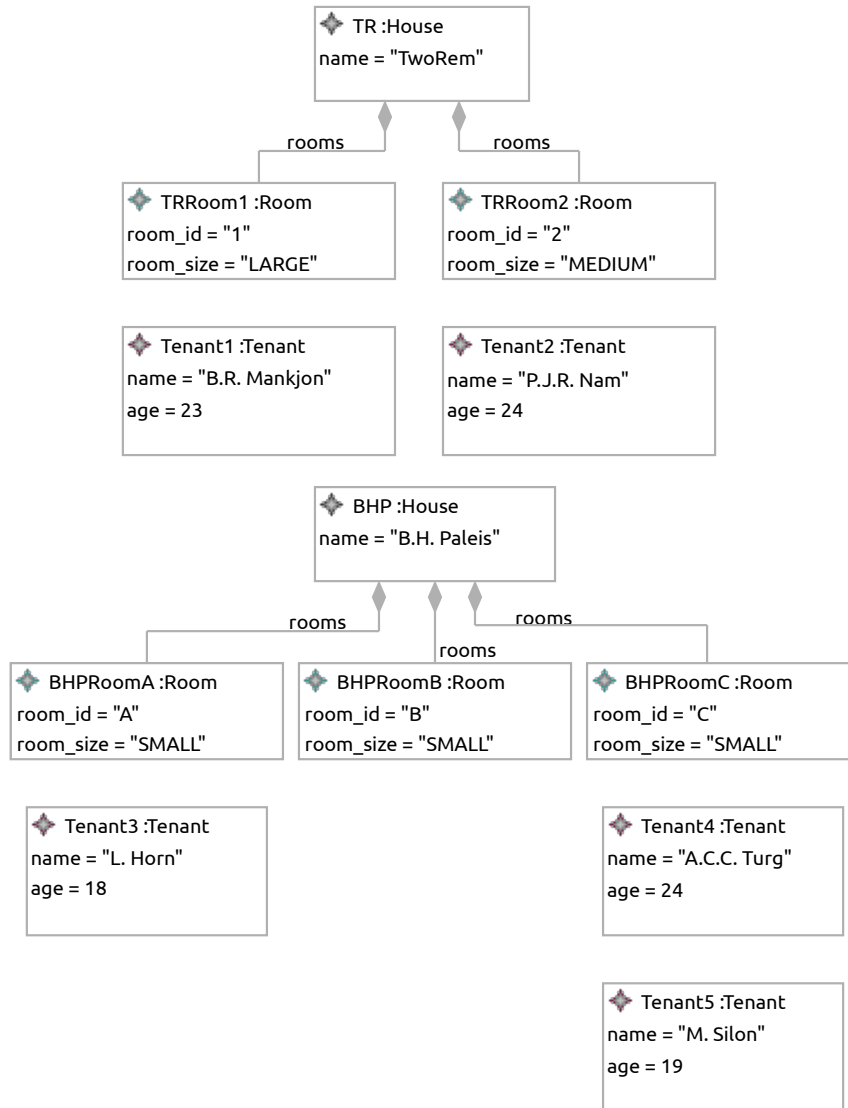
(a) Instance Model Im_{10}
