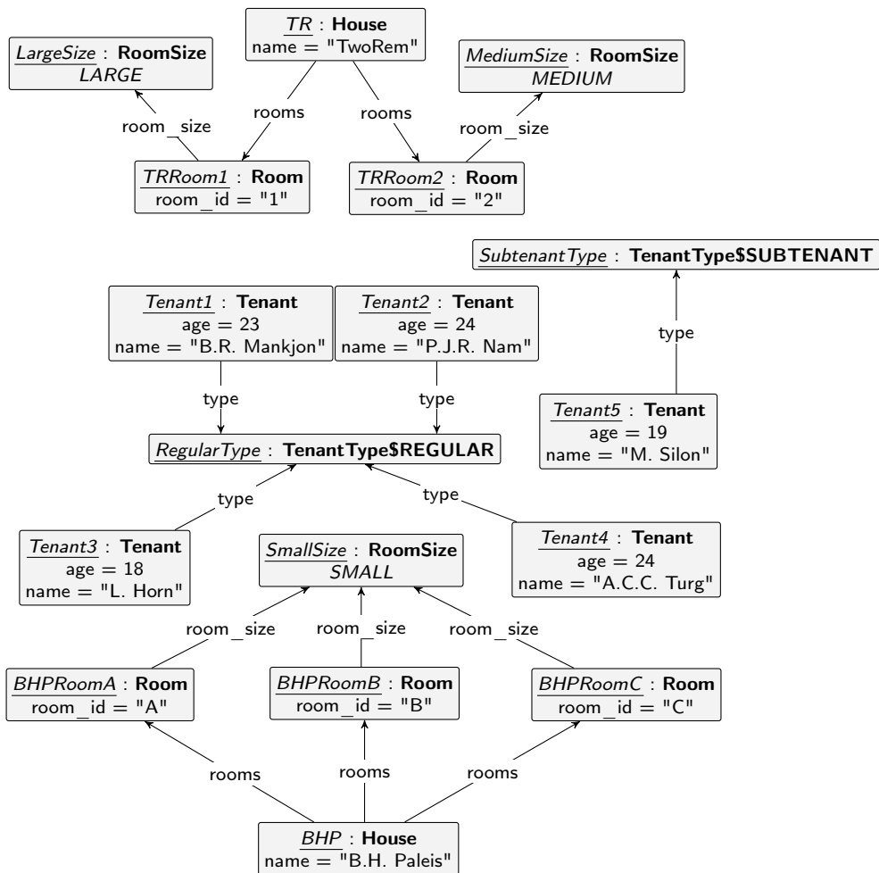
(a) Instance Graph IG_{12}
