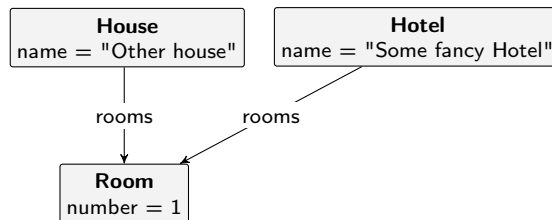
Figure 3.16: Invalid instance graph with multiple containments for the Room-typed node
