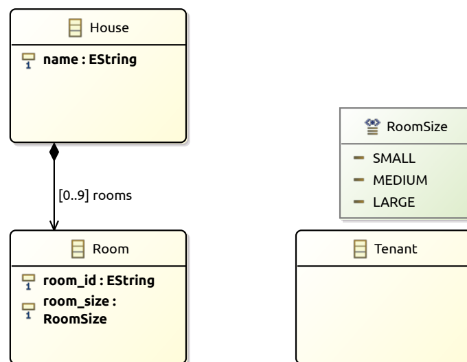
(b) Type Model Tm_8
