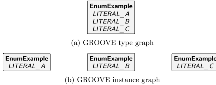
Figure 4.3: Encoding of the EnumExample enumeration type as one type with multiple flags
