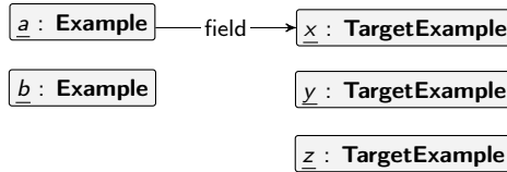
(b) IG_{NullableClassField} with examples of different nodes with different values for field
