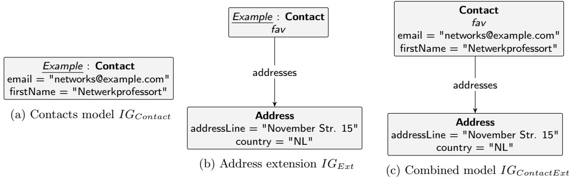
Figure 4.12: Example of the combination of instance graphs
