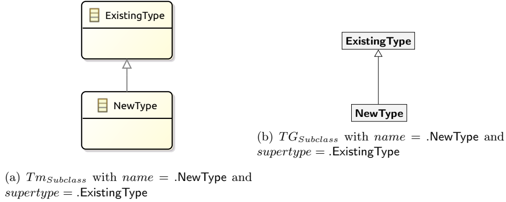
Figure 5.3: Visualisation of the transformation of regular subclasses
