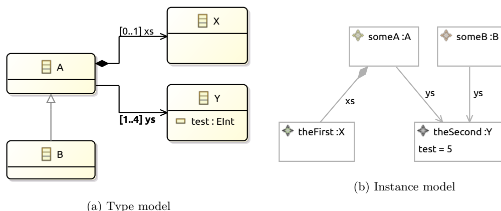
Figure 2.2: Examples of different models in Ecore
