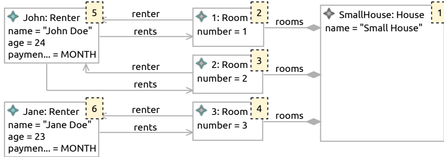
(a) Instance model based on Ecore notation
