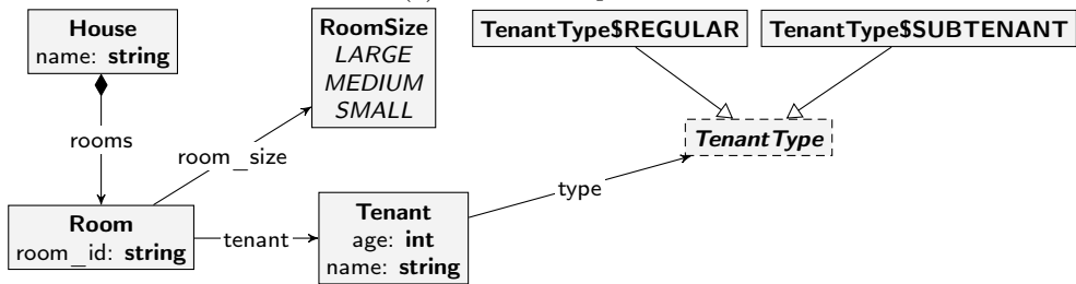
(b) Type Graph TG_{13}
