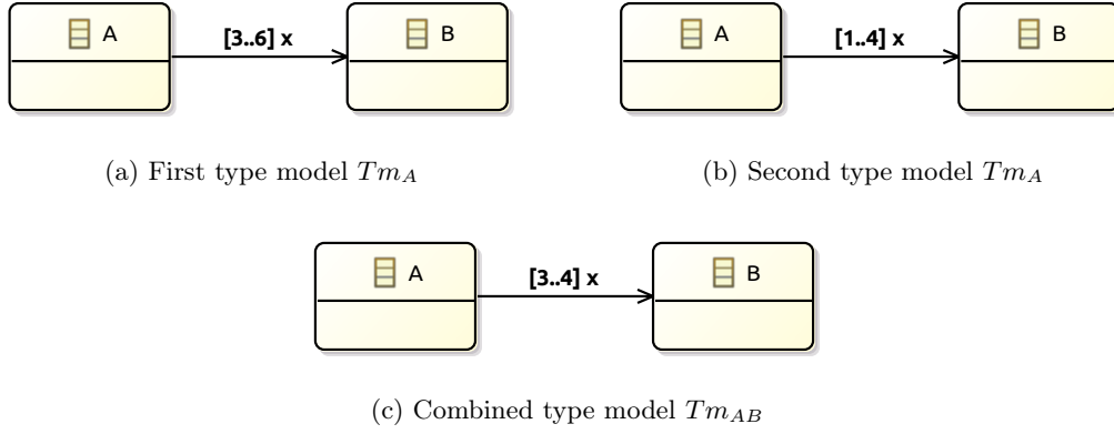
Figure 4.6: Combination of field signatures when field is present in both type models
