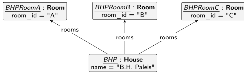
(a) Instance Graph IG_5
