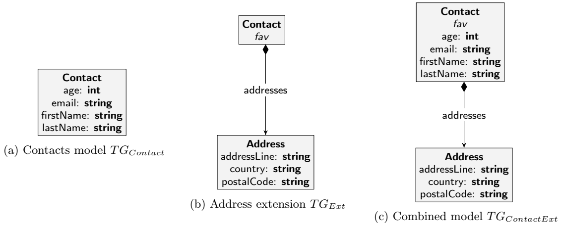
Figure 4.9: Example of the combination of type graphs
