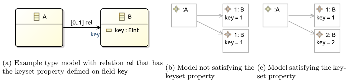
Figure 3.7: Examples of the keyset property.
