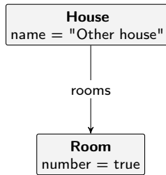
Figure 3.13: Invalid instance graph with improper type for the target of edge number
