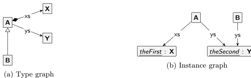
Figure 2.3: Examples of different graphs in GROOVE
