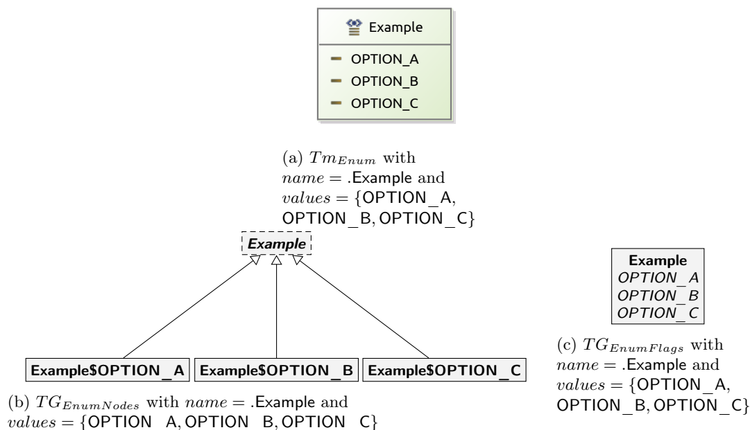
Figure 5.4: Visualisations of the transformations of enumeration types
