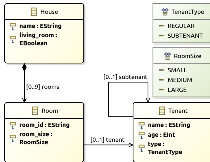
(b) Type model
