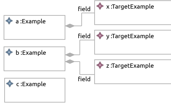
(a) Im_{ContainedClassSetField} with examples of different nodes with different values for field
