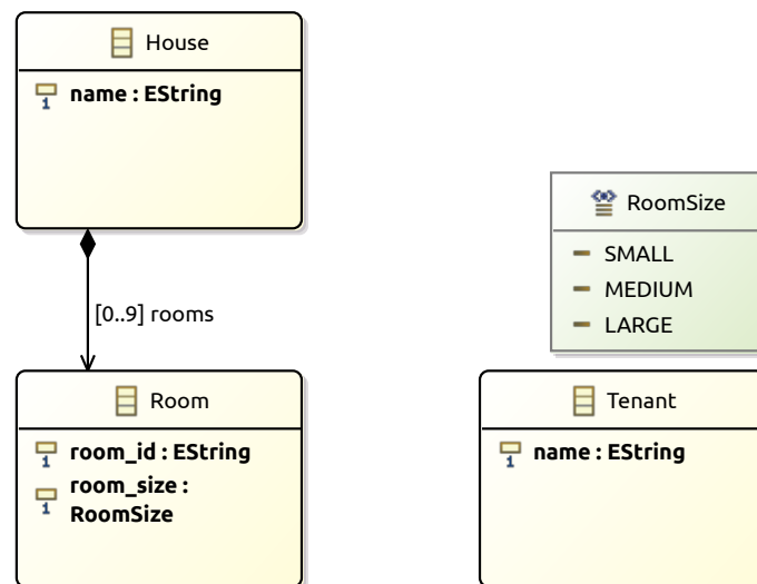
(b) Type Model Tm_9
