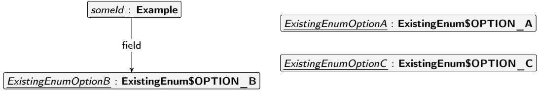
(b) IG_{EnumFieldNodes} with one node and its edge referencing enumeration option OPTION\_B
