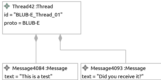
(a) The chat application instance model Im_{Chat}
