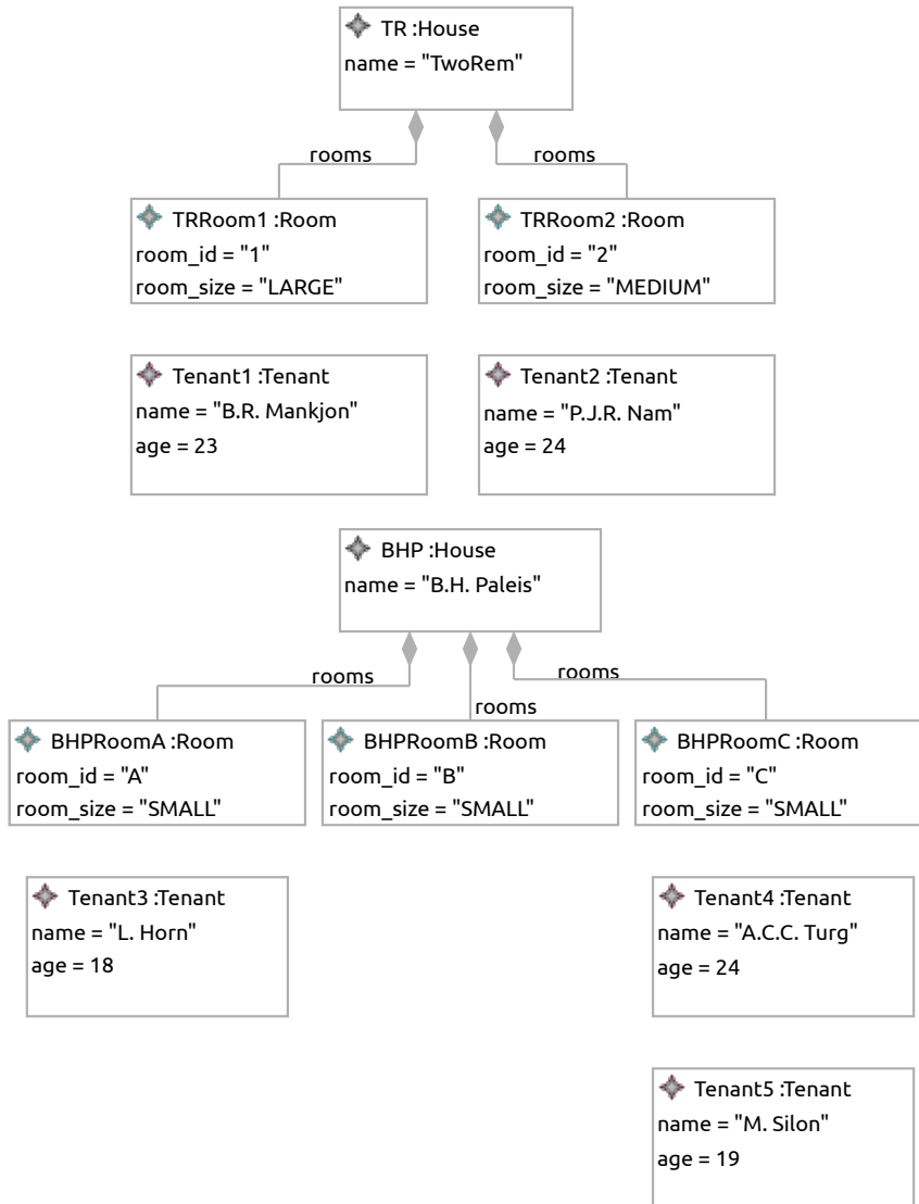
(a) Instance Model Im_{11}
