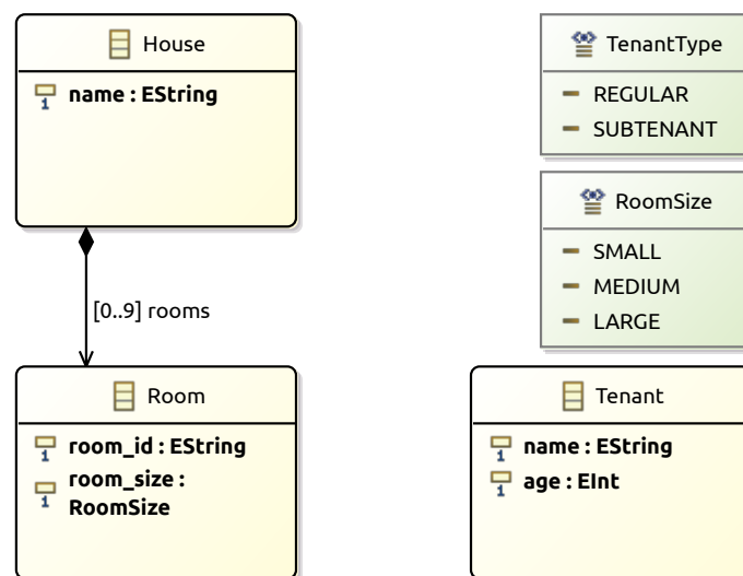
(b) Type Model Tm_{11}
