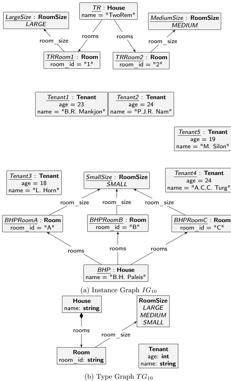
Figure 6.21: The GROOVE graphs after step 10
