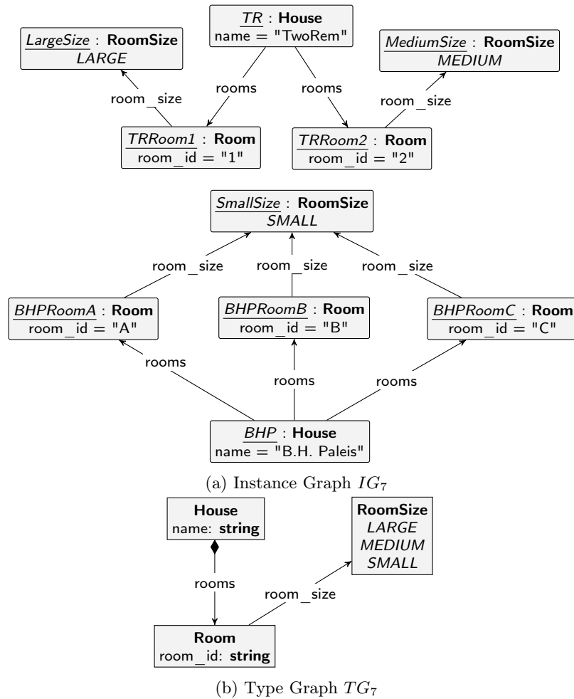
Figure 6.15: The GROOVE graphs after step 7
