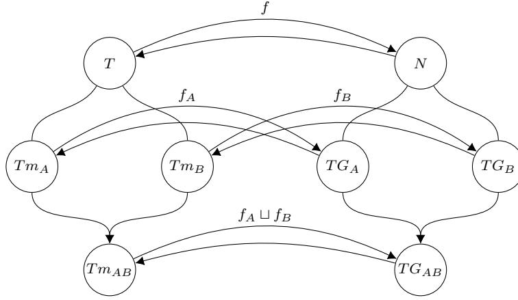
Figure 4.5: Structure for transforming between type models and type graphs
