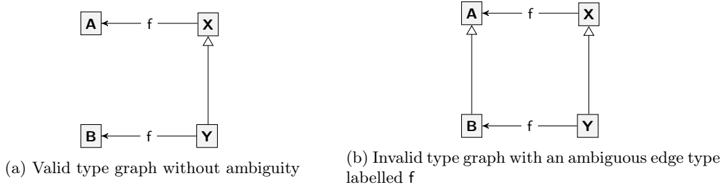
Figure 3.10: Example of ambiguity within edge types
