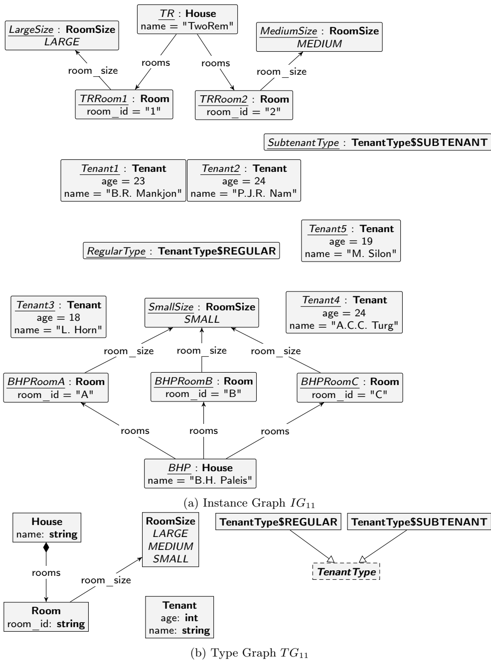
Figure 6.23: The GROOVE graphs after step 11
