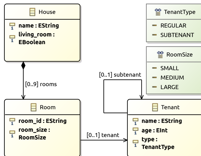
(b) Type Model Tm_{15}
