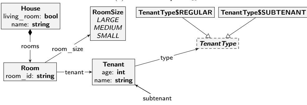
(b) Type Graph TG_{15}
