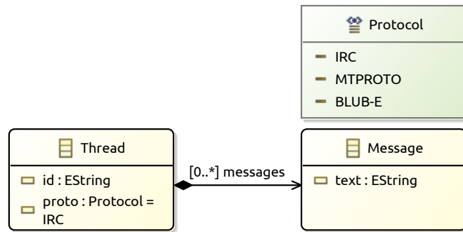
(a) The chat application model Tm_{Chat}
