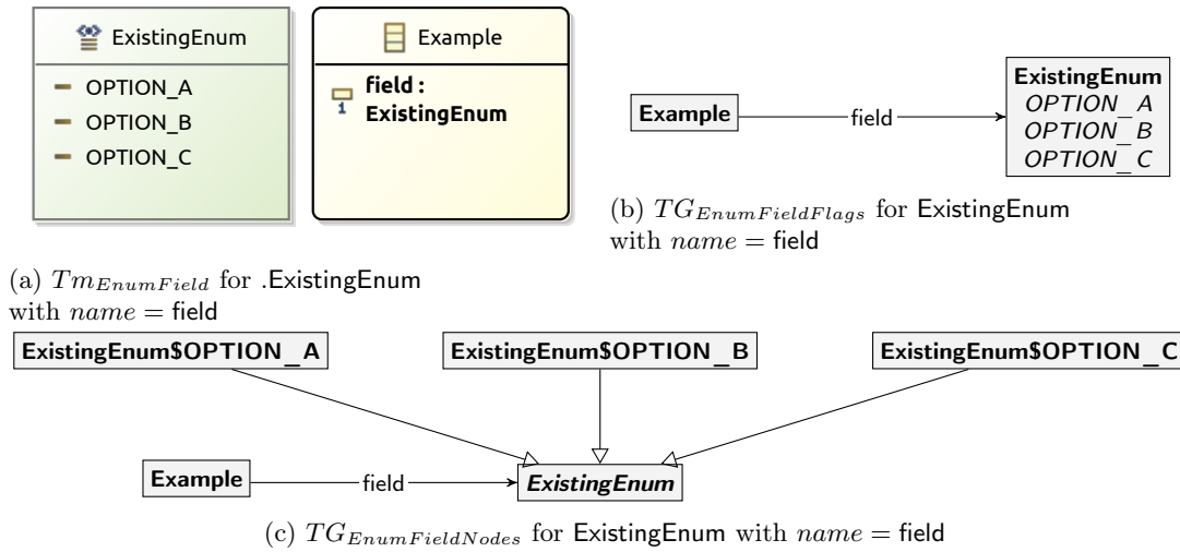
Figure 5.7: Visualisation of the transformation of a field typed by an enumeration type
