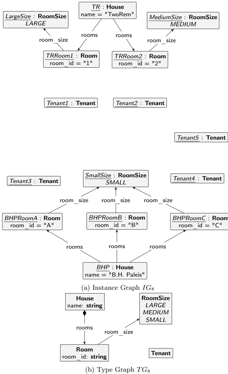
Figure 6.17: The GROOVE graphs after step 8
