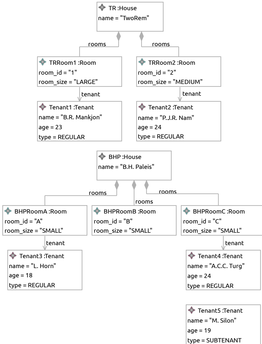
(a) Instance Model Im_{13}
