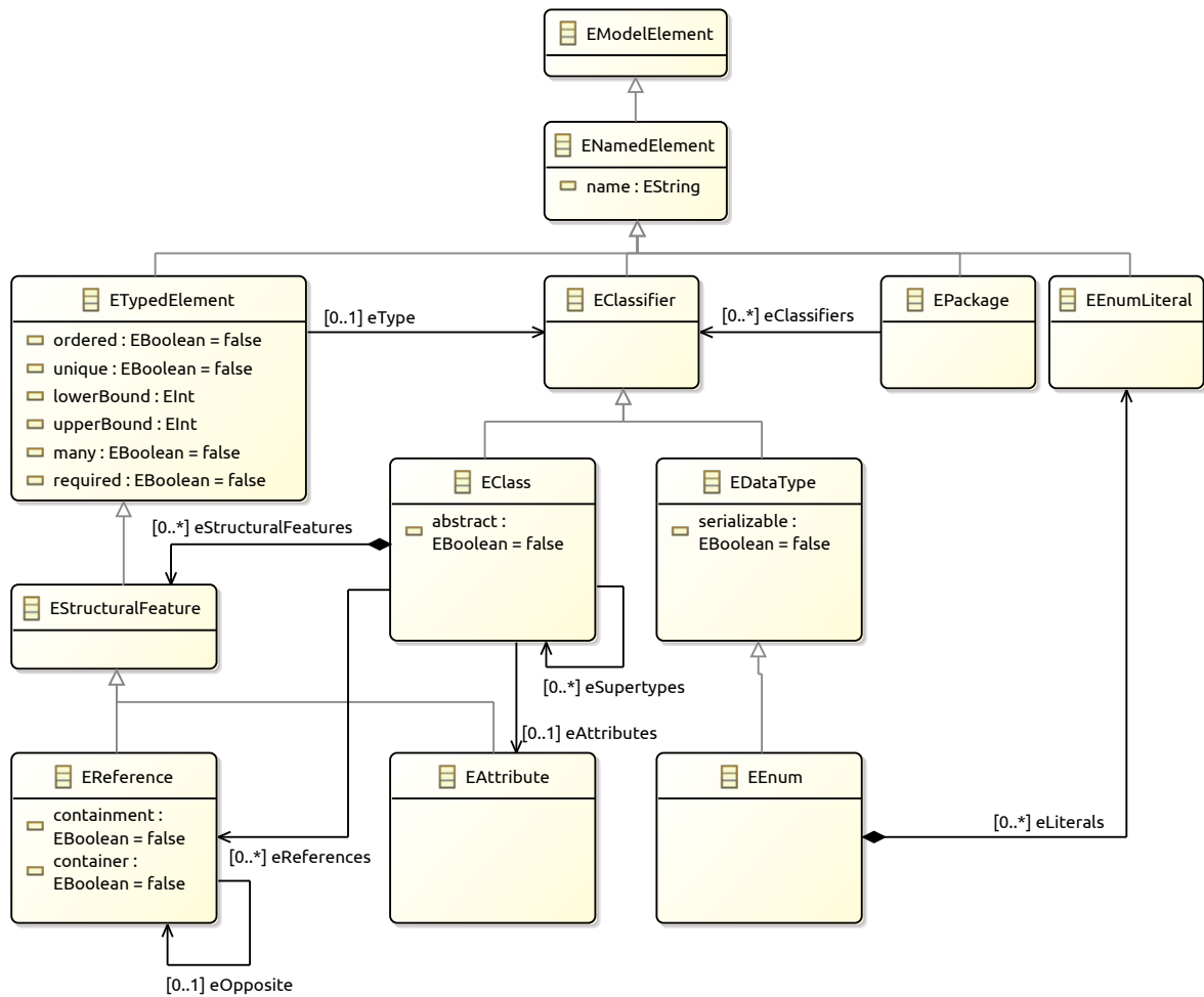
Figure 2.1: Simplified version of the Ecore metamodel
