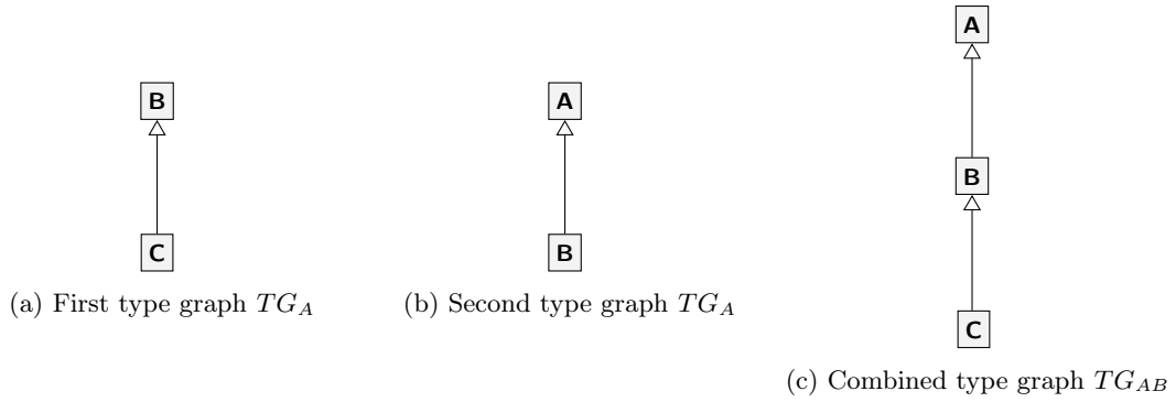
Figure 4.8: Combination of the inheritance relation
