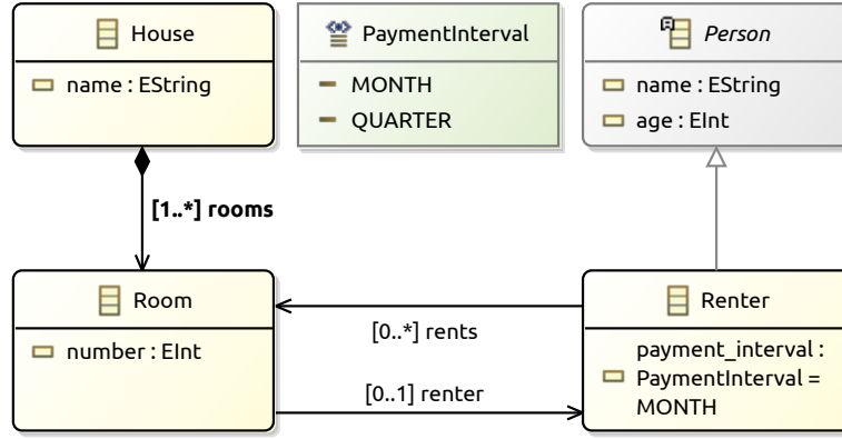
(a) Type model in Ecore notation
