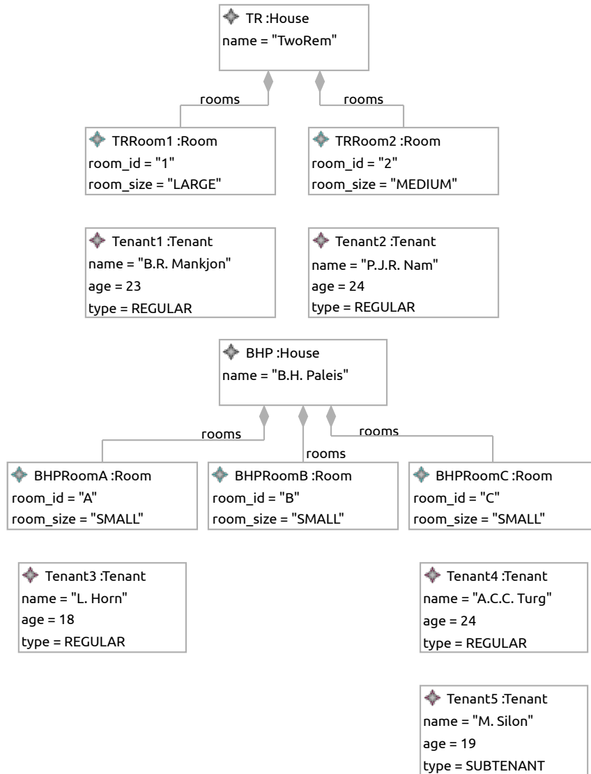
(a) Instance Model Im_{12}
