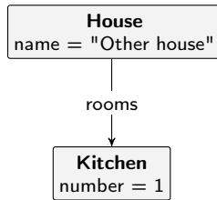
Figure 3.12: Invalid instance graph with improper node types
